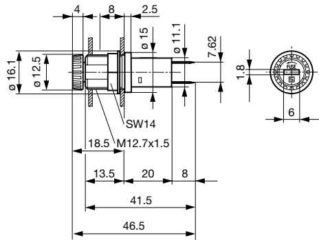
Variants Fingergrip 3101.0025 and 3101.0225
