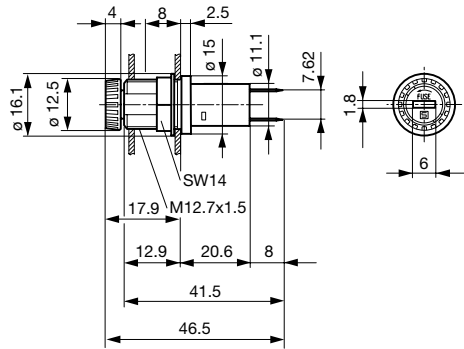
Variants Fingergrip 3101.0125 and 3101.0325
