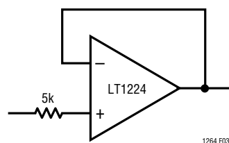
Figure 3. Wideband Buffer
