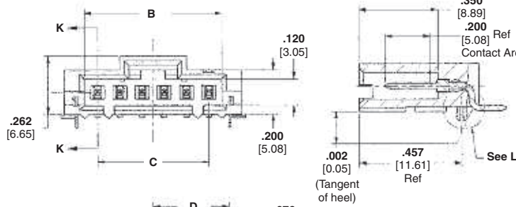
Section K-K
