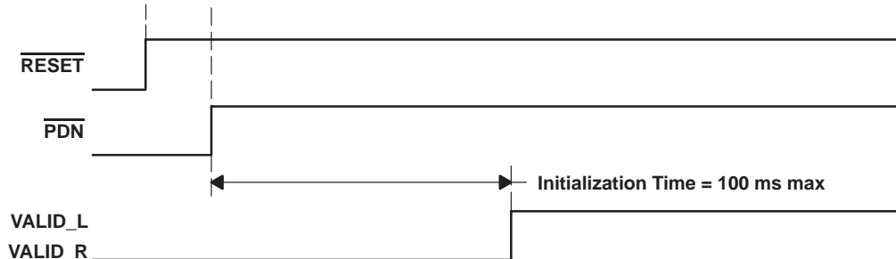
Figure 1. Power-Up Timing ( \overline{\text{RESET}} Preceding PDN)
