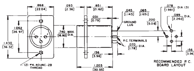
(Component Side)
