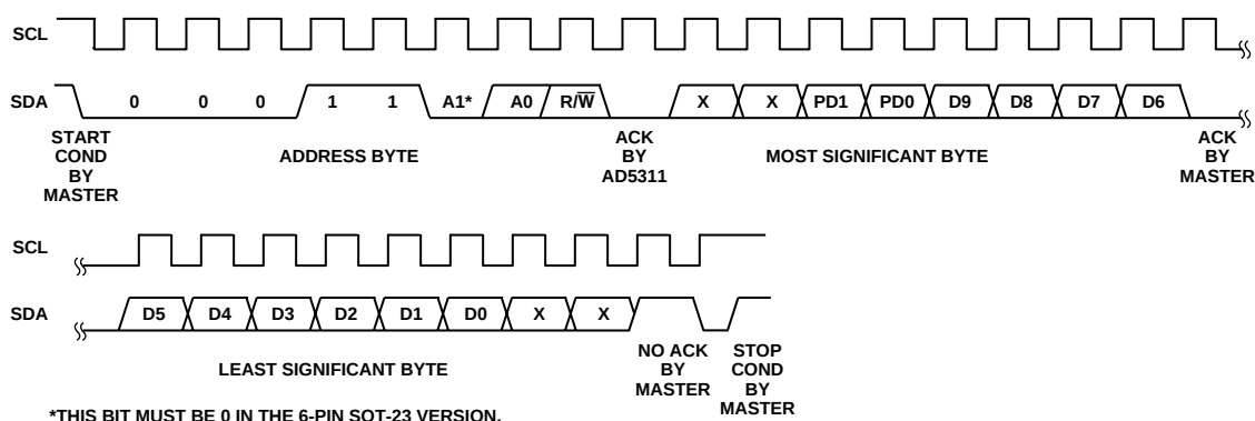
Figure 28. AD5311 Readback Sequence
