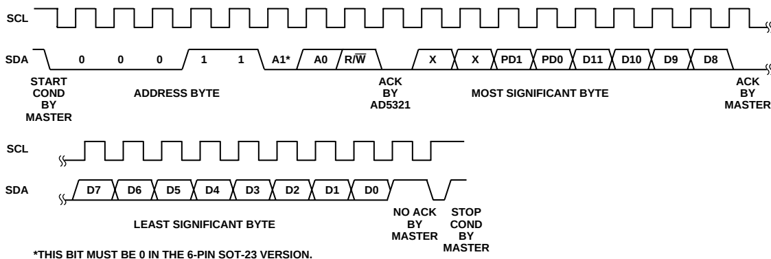
Figure 29. AD5321 Readback Sequence
