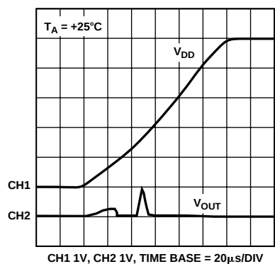
Figure 17. Power-On Reset to 0 V
