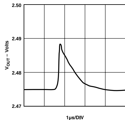
Figure 19. Major-Code Transition
