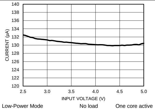
Figure 5. Low-Power PFM Mode Current Consumption vs V_{IN}
