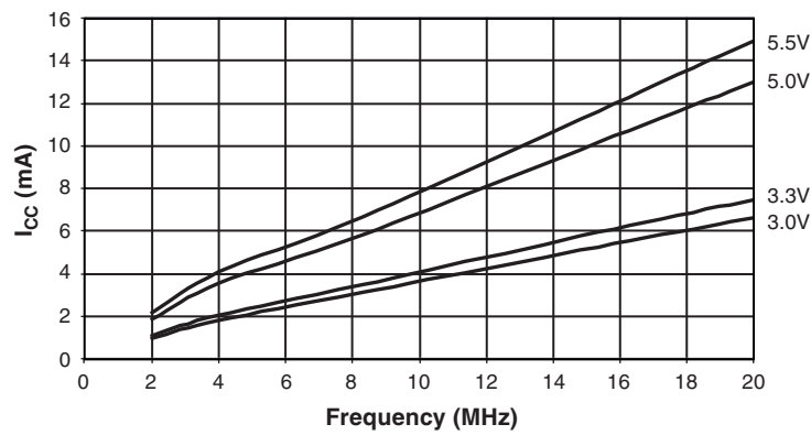
Figure 2-1. Active Supply Current versus Frequency (1MHz to 20MHz)
