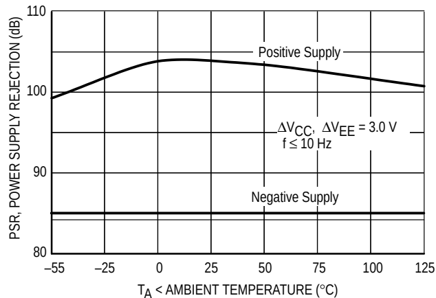
Figure 24. Power Supply Rejection versus Temperature
