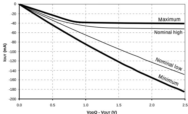
Figure 10: Pull-Up Characteristics
