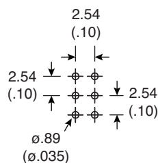
P.C. Mounting
