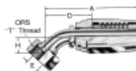
ORS Swivel 45° Elbow FJ9725-
