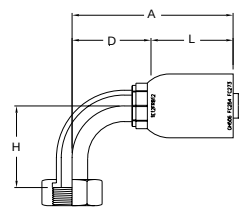
ORS® Swivel 90° Elbow
