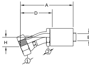
SAE 37° (JIC) swivel FC5963/FJ9775 22 1/2° elbow FC5965/FJ9776 30° elbow FC9627/FJ9777 45° elbow
