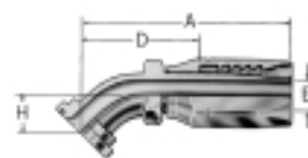
Code 61 SAE J518 45° split flange FC5138-
