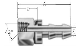
SAE 42° inverted female flare 4743-
