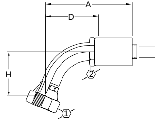
SAE 37° (JIC) swivel FC5967/FJ9778 60° elbow FC5969/FJ9779 67 1/2° elbow
