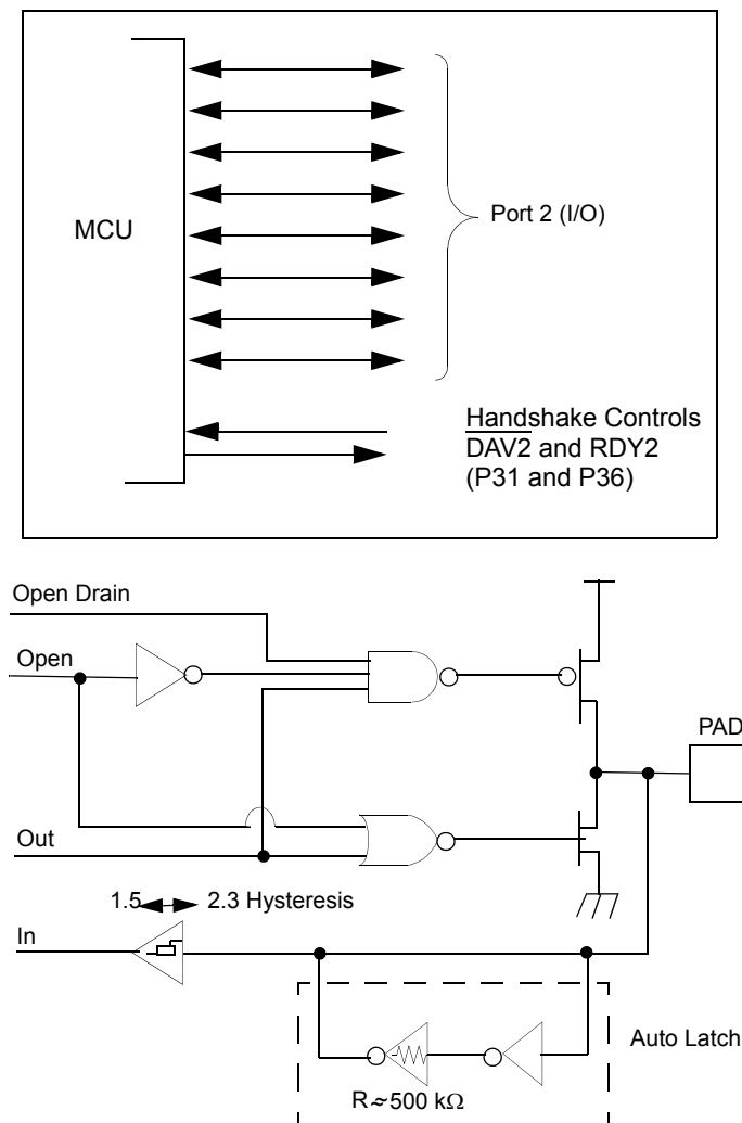
Figure 20. Port 2 Configuration
