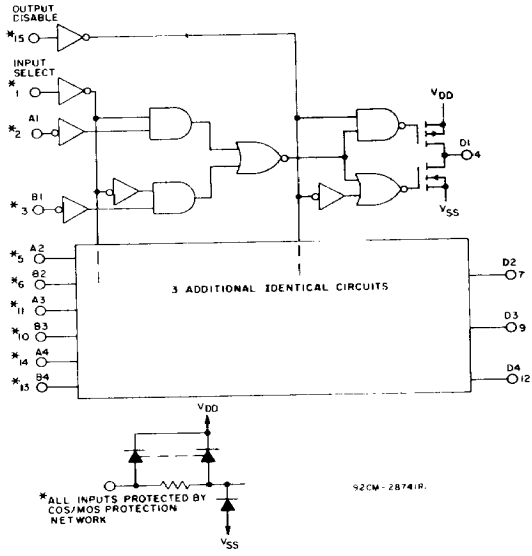
Fig. 1 - Logic diagram for CD40257B.
