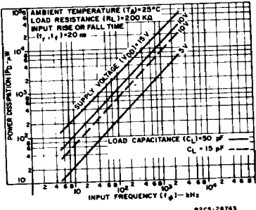
Fig.8 - Typical dynamic power dissipation as a function of input frequency (one INPUT to one OUTPUT).
