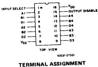
TERMINAL ASSIGNMENT
