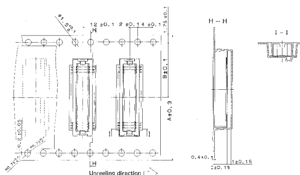
(50 contacts)
