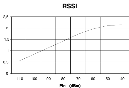
Figure 12. RSSI Voltage
