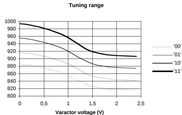
Figure 7. RF Frequency vs. Varactor Voltage and VCO Frequency bit ( V_{\text{DD}} = 2.25\text{V} )
