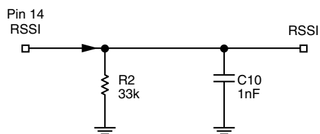
Figure 13. RSSI Network
