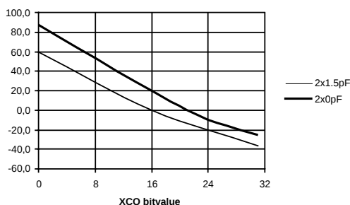
Figure. 21 XCO Tuning
