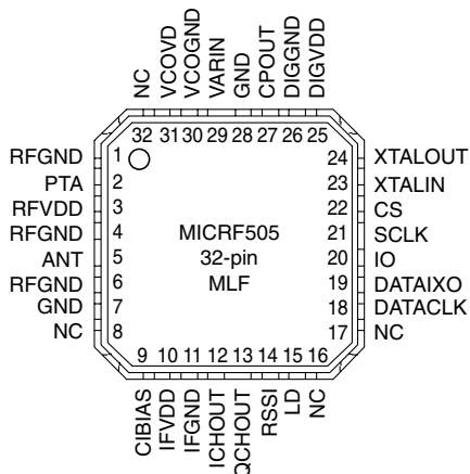
32-Pin MLF™
