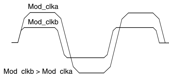
Figure 16. Two Different Modulator Clock Settings
