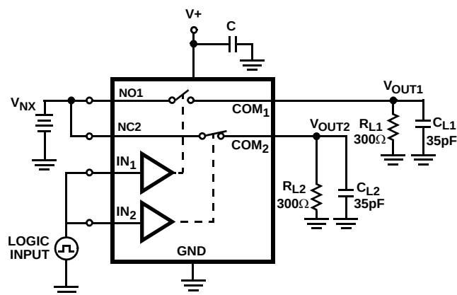
FIGURE 3B. TEST CIRCUIT (ISL8325 ONLY)
