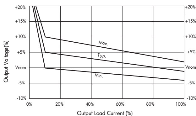
Graph 1: Load regulation
