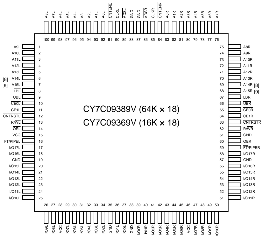
Figure 2. 100-pin TQFP pinout (Top View)
