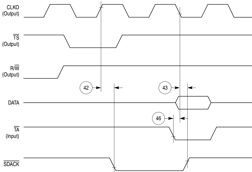
Figure 47. \overline{\text{SDACK}} Timing Diagram—Peripheral Write, Externally-Generated \overline{\text{TA}}
