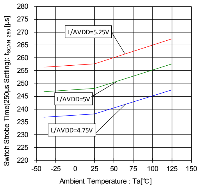
Figure 115. Switch Strobe Time- Temperature Characteristic (250μs Setting)
