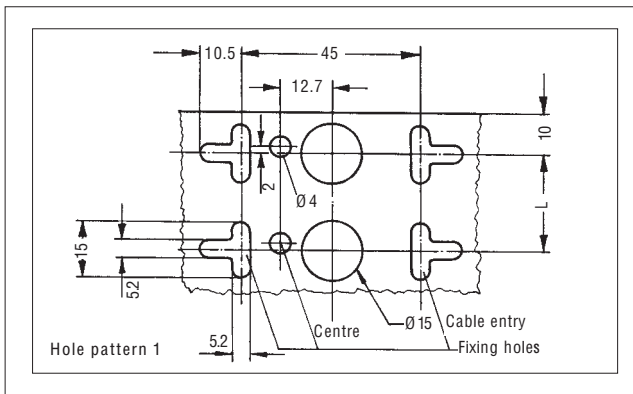
■ Examples of back-mount frames for the LSA-PLUS series 2/8
