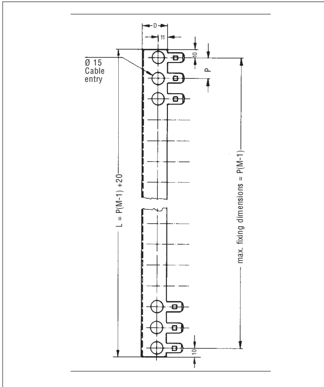
■ Examples of back-mount frames for the LSA-PLUS series 2/10
