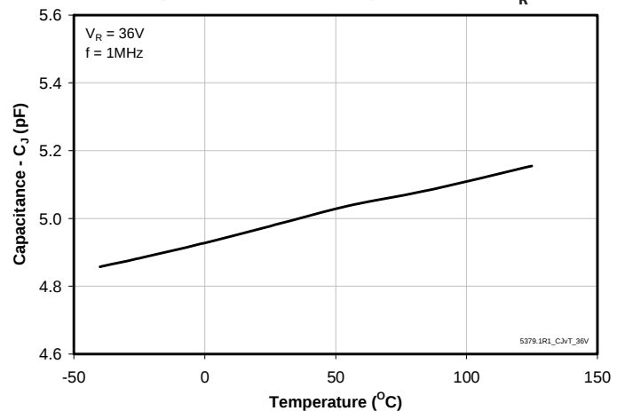
Junction Capacitance vs. Temperature at V_R = 36\text{V}
