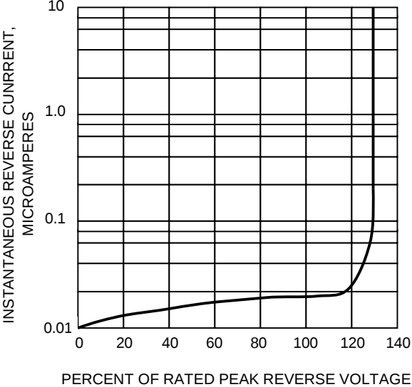
FIG.2-TYPICAL REVERSE CHARACTERISTICS
