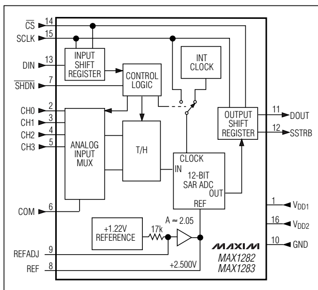
Figure 3. Functional Diagram
