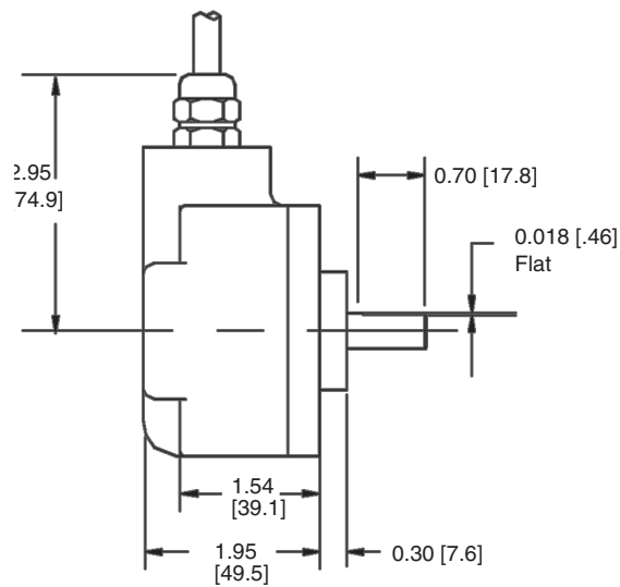
Cable Exit
