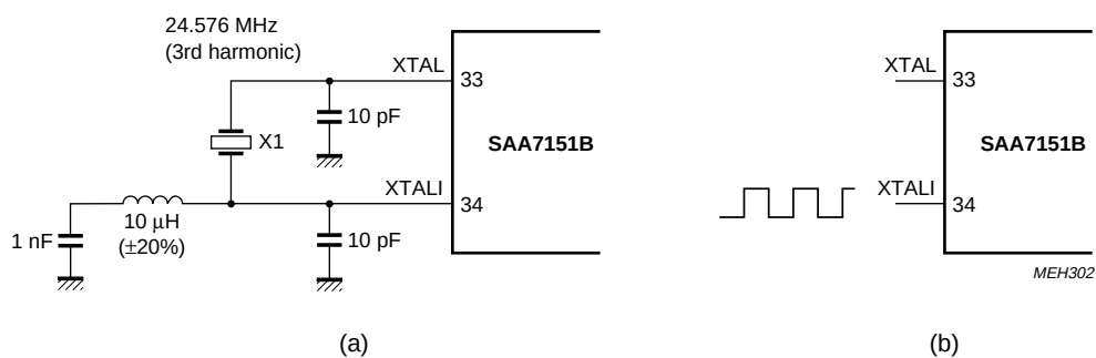
Fig.18 Oscillator application (a) and optional clock from external (b).
