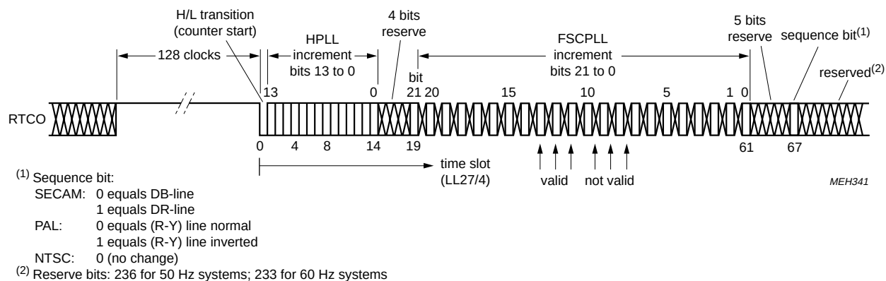
Fig.11 RTCO timing.
