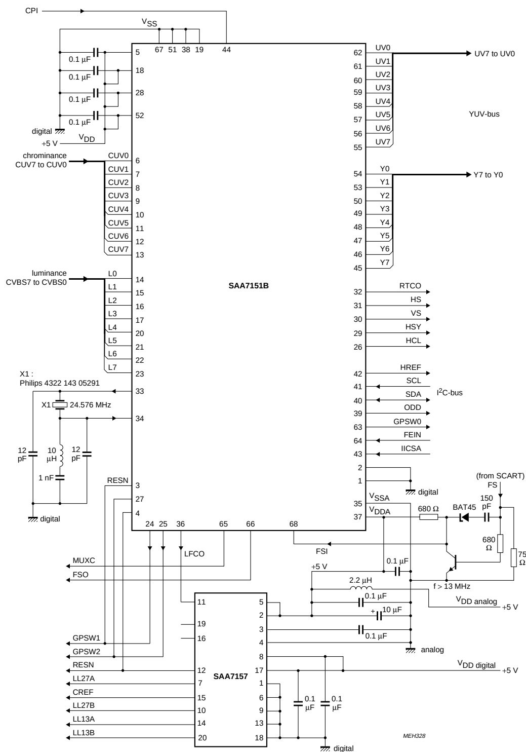
Fig.19 Application of SAA7151B.
