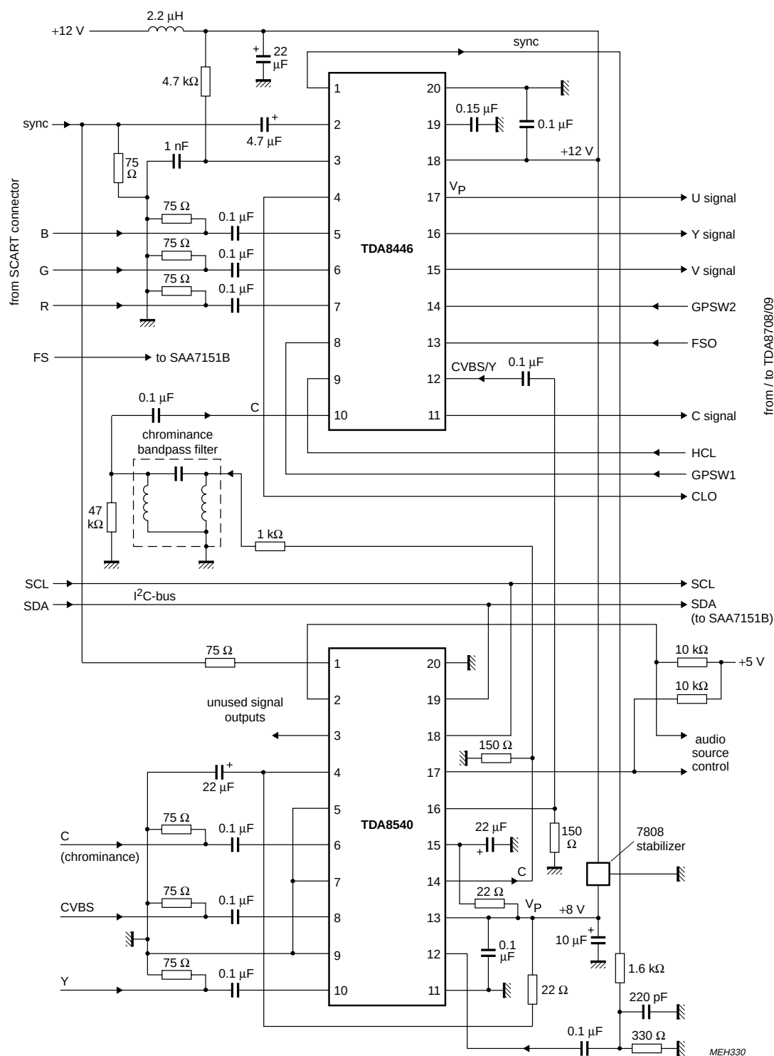
Fig.20 Application of input signal selecting (SCART interface).
