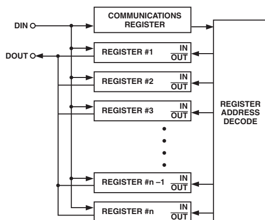
Figure 41. Addressing ADE7759 Registers via the Communications Register
