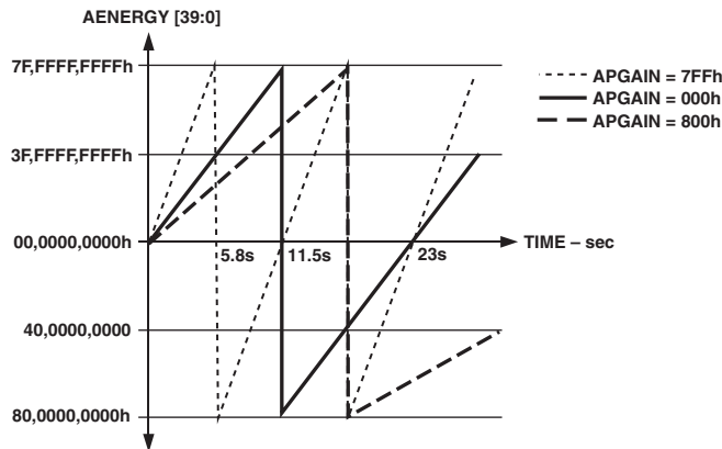
Figure 37. Energy Register Rollover Time for Full-Scale Power (Minimum and Maximum Power Gain)
