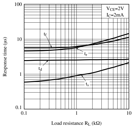
Fig.12 Response Time vs. Load Resistance (active region)
