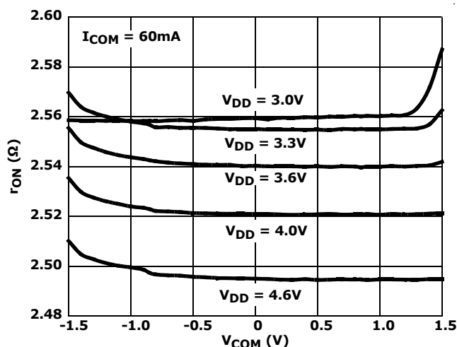
FIGURE 9. AUDIO ON-RESISTANCE vs SUPPLY VOLTAGE vs SWITCH VOLTAGE
