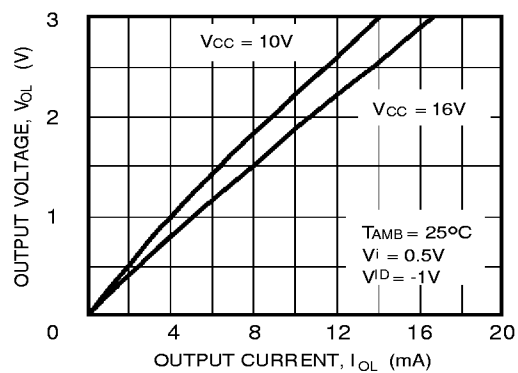
Figure 3b : Low Level Output Voltage versus Low Level Output Current
