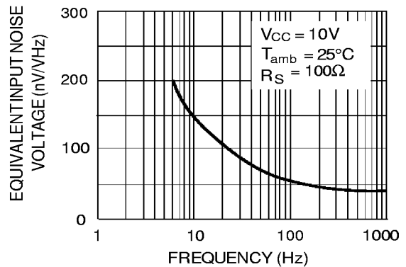
Figure 10 : Input Voltage Noise versus Frequency
