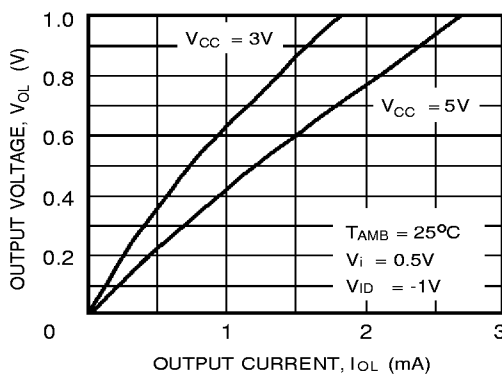
Figure 3a : Low Level Output Voltage versus Low Level Output Current
