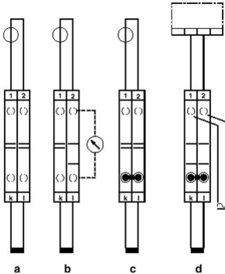
Simple current transformer test circuit
