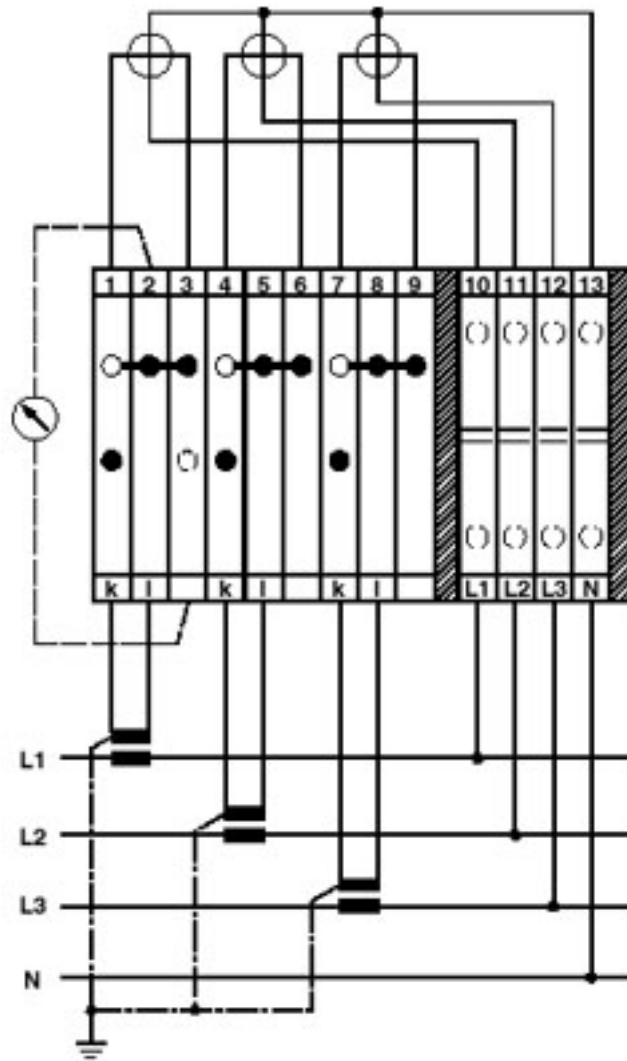
Meter test set (active current) constructed with UGSK and URTK-BEN
