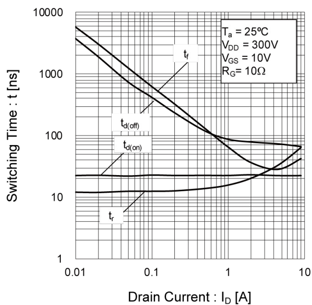
Fig.19 Switching Characteristics
