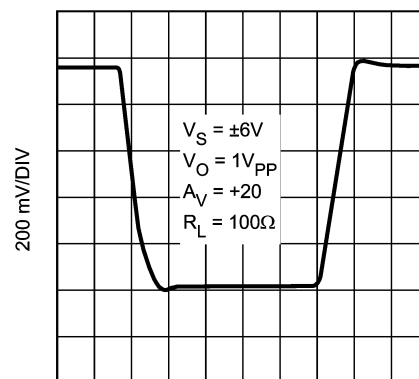
Non-Inverting Large Signal Pulse Response
