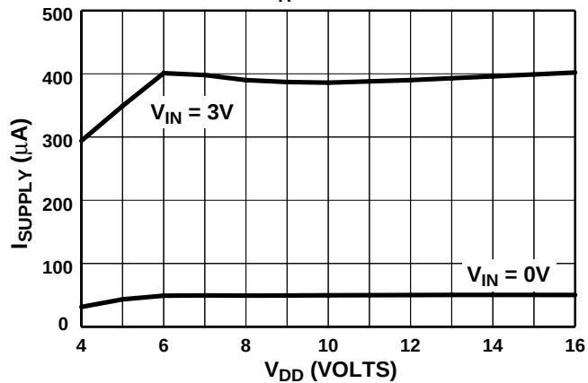
Quiescent Supply Current vs. Supply Voltage T_A = 25^\circ\text{C}
