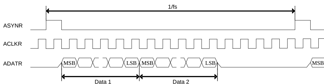
FIGURE 31. ACLKMASTER=0, RM_SYNC=1
