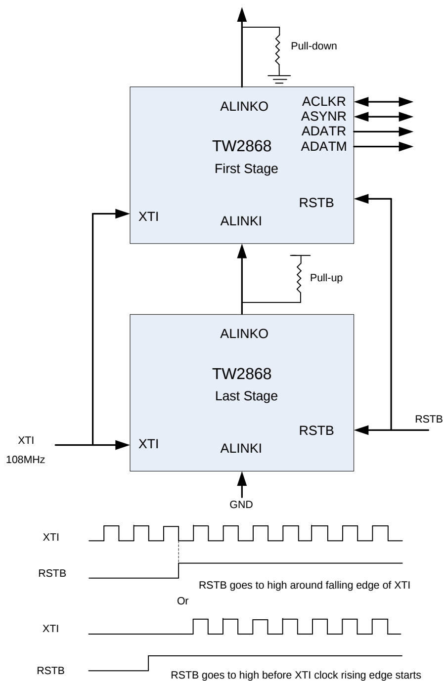
FIGURE 26. RSTB TIMING ON XTI 108MHZ MODE
