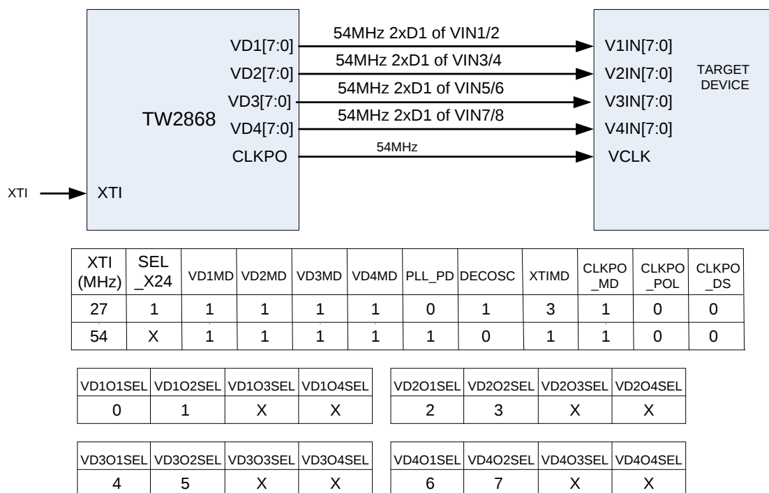
FIGURE 19. 4X2D1 WITH 54MHZ CLOCK VIDEO OUTPUT INTERFACE WHEN TARGET HAS ONLY ONE CLOCK INPUT
