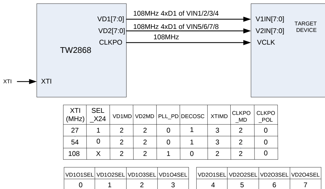
FIGURE 18. 2X4D1 WITH 108MHZ CLOCK VIDEO OUTPUT INTERFACE WHEN TARGET HAS ONLY ONE CLOCK INPUT
