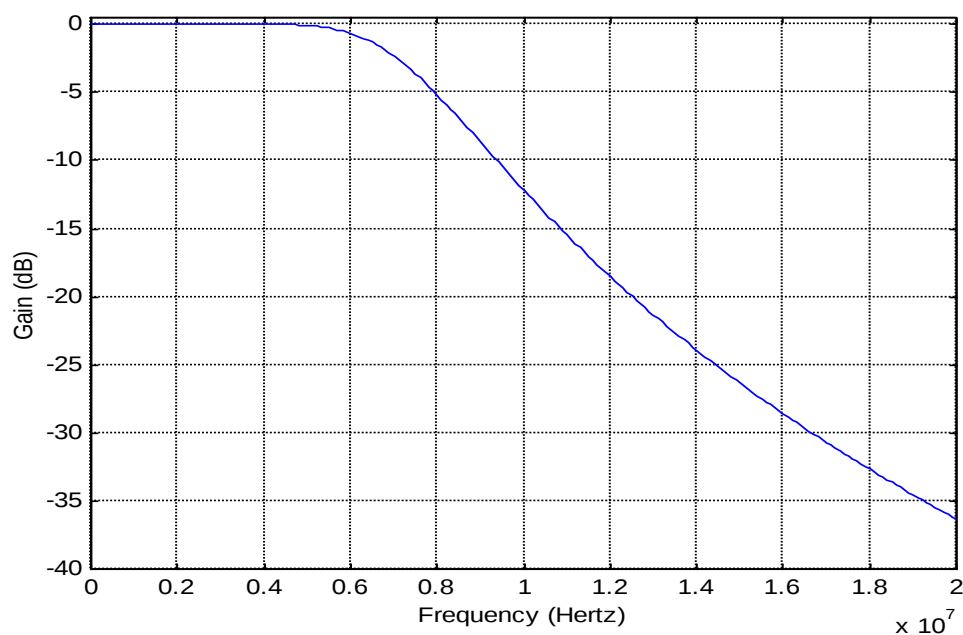
FIGURE 1. THE FREQUENCY RESPONSE OF ANTI-ALIASING FILTER
