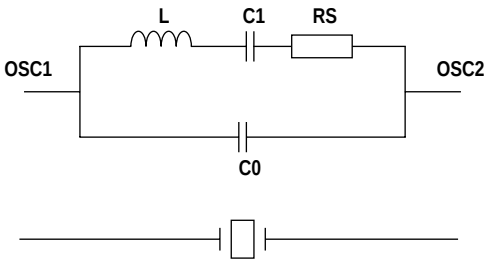
(b) Crystal equivalent circuit
