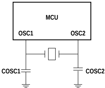
(a) Crystal/ceramic resonator oscillator connections
