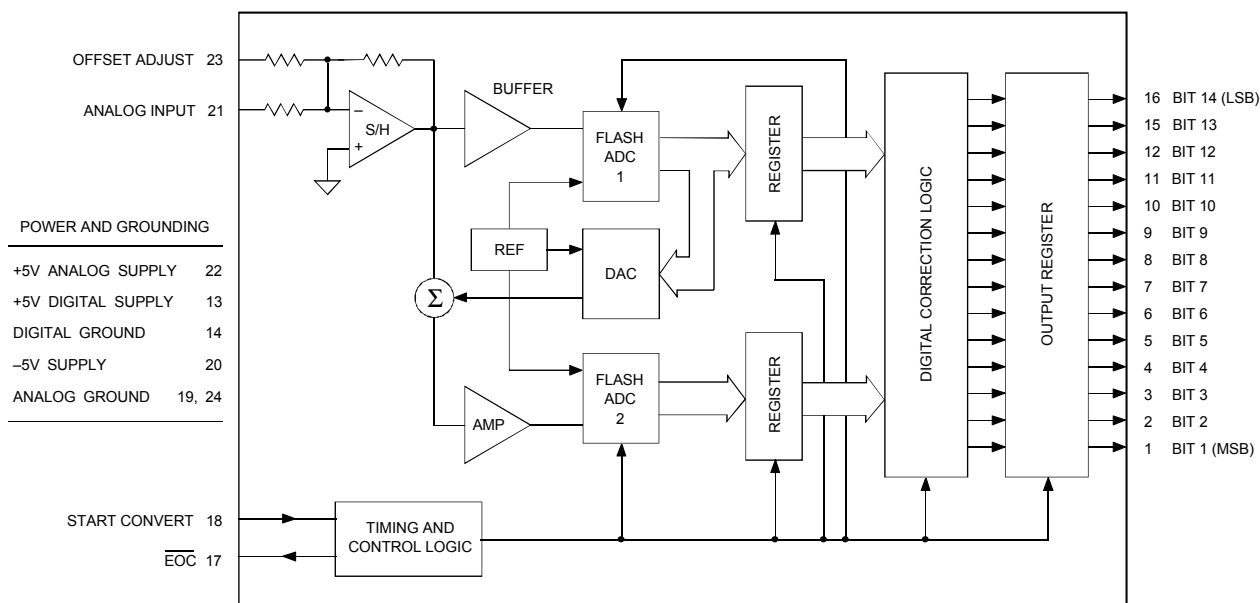
Figure 1. ADS-943 Functional Block Diagram
