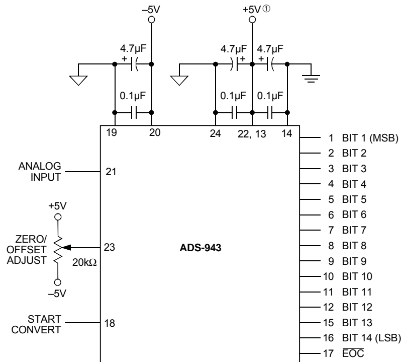
Figure 3. Connection Diagram
