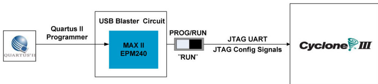
Figure 4-1. The JTAG configuration scheme
