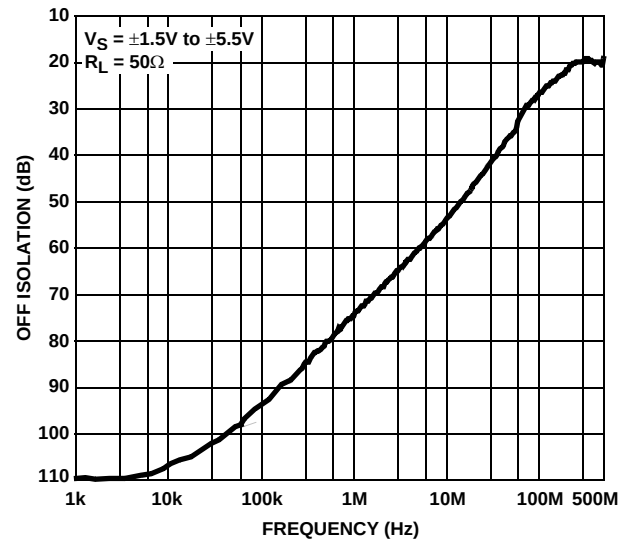
FIGURE 16. OFF ISOLATION
