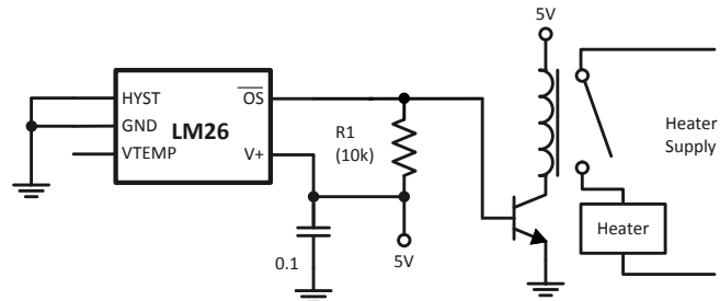
Figure 13. Simple Thermostat
