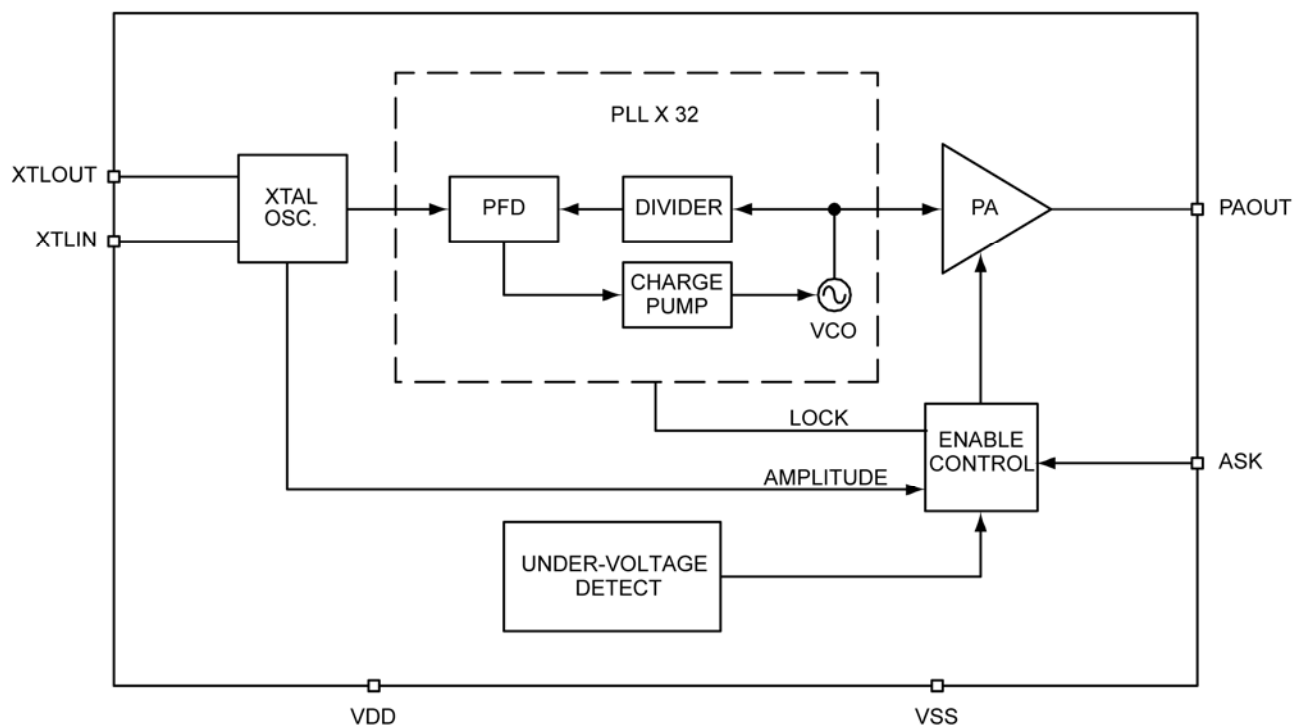
Figure 3. MICRF113 Functional Block Diagram
