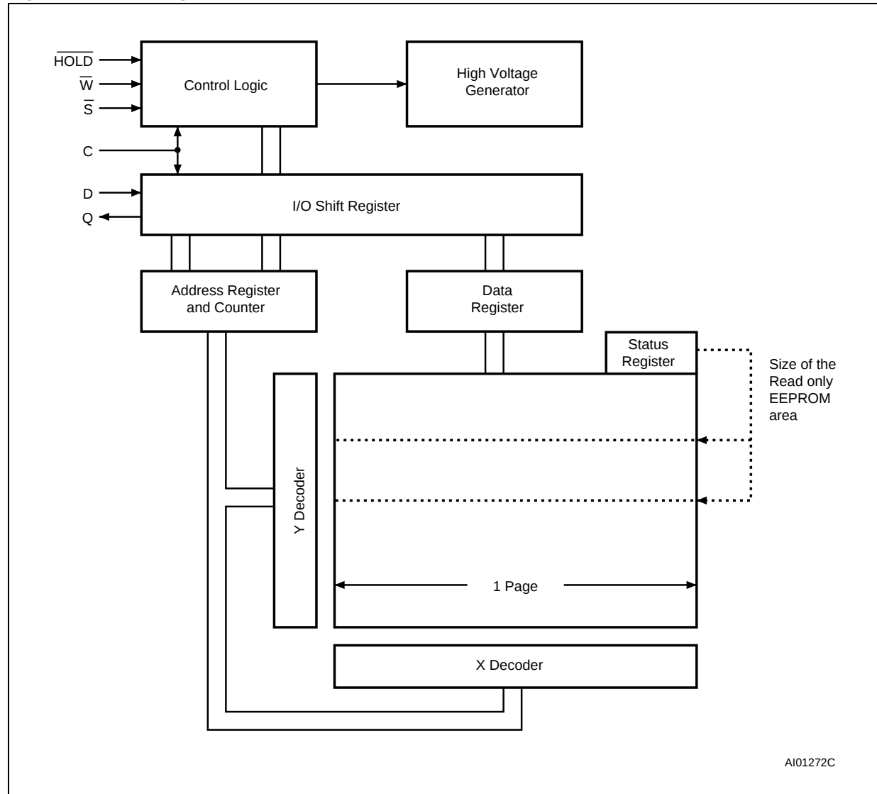
Figure 7. Block Diagram
