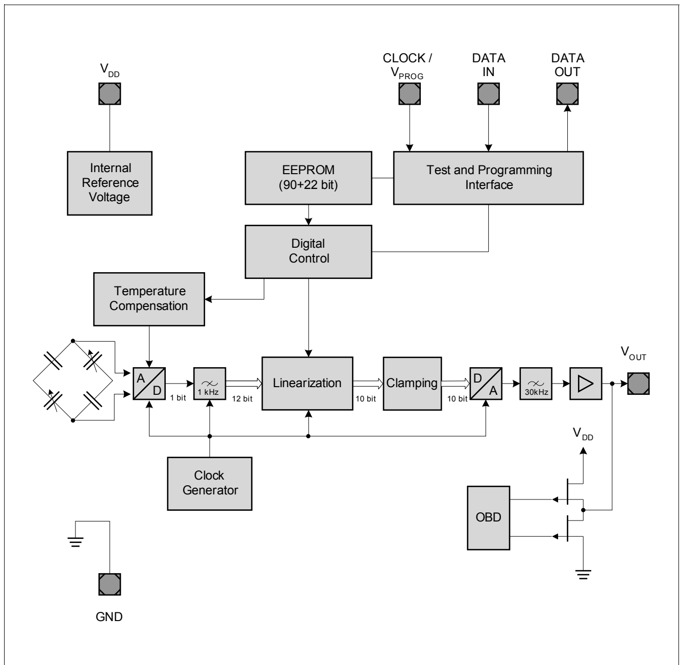
Figure 2 Block Diagram 1)
