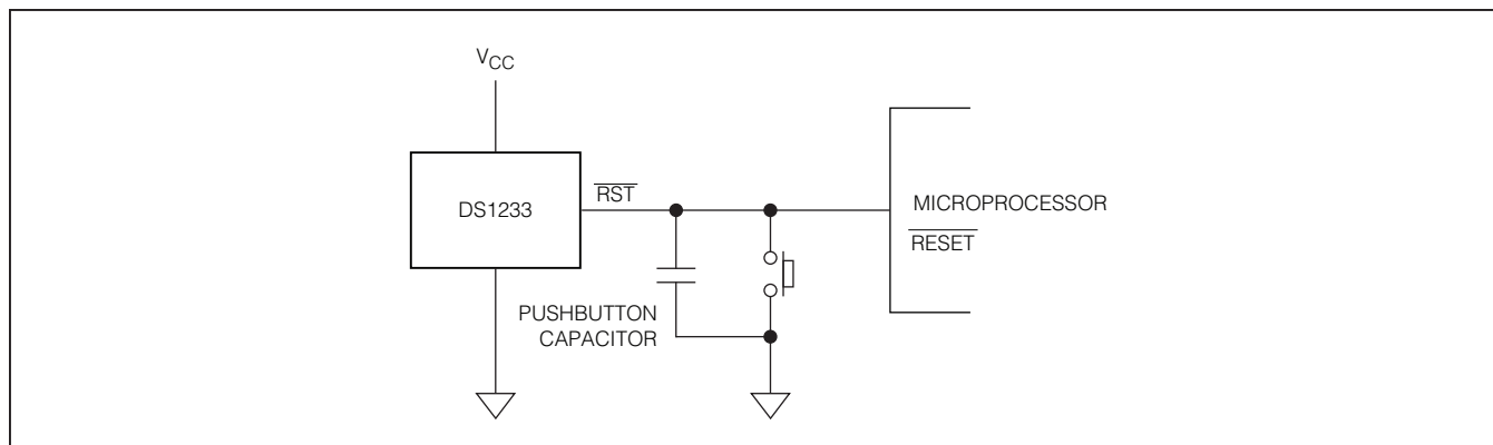
Figure 2. Application Example
