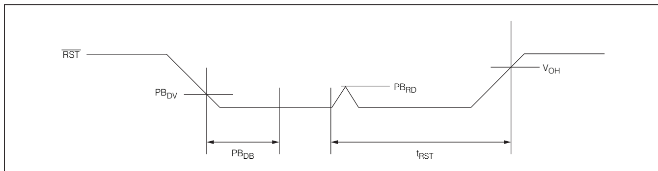
Figure 3. Pushbutton Reset
