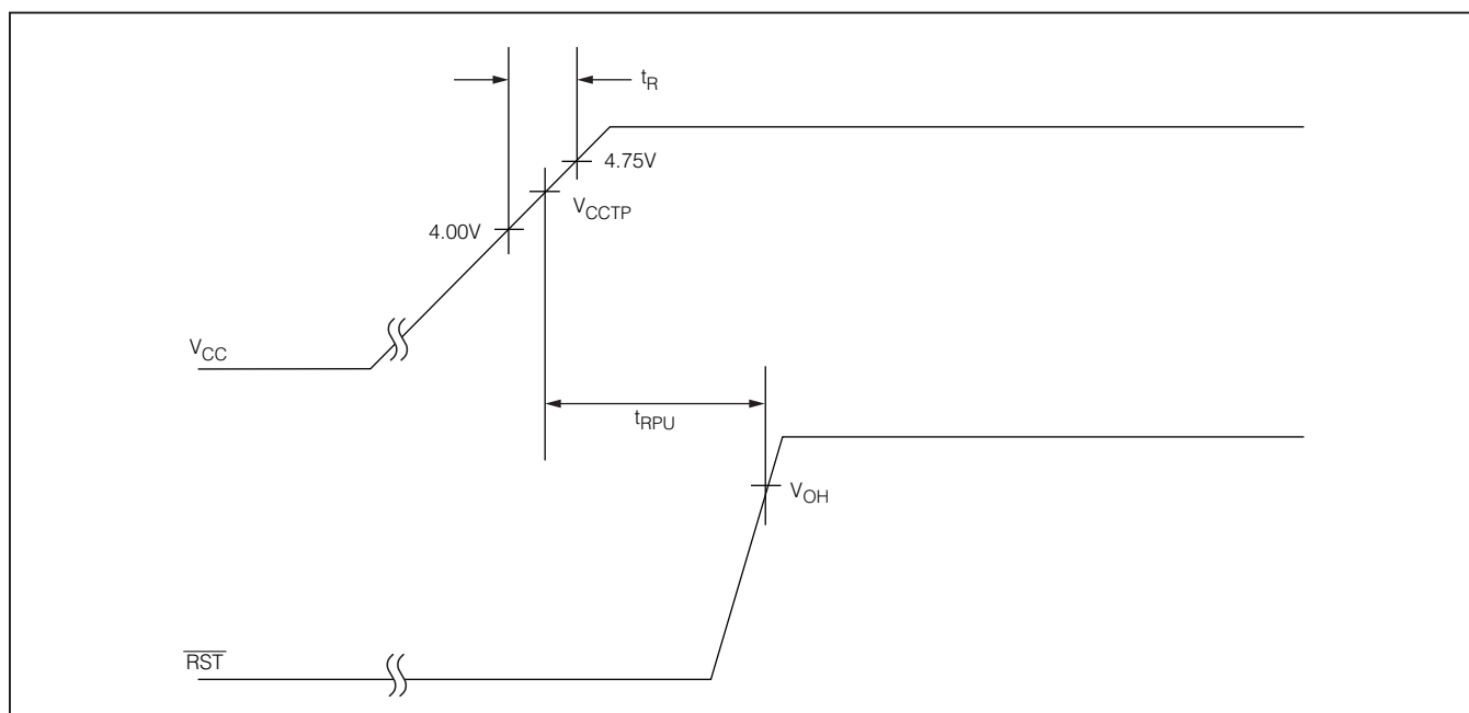
Figure 4. Power Up
