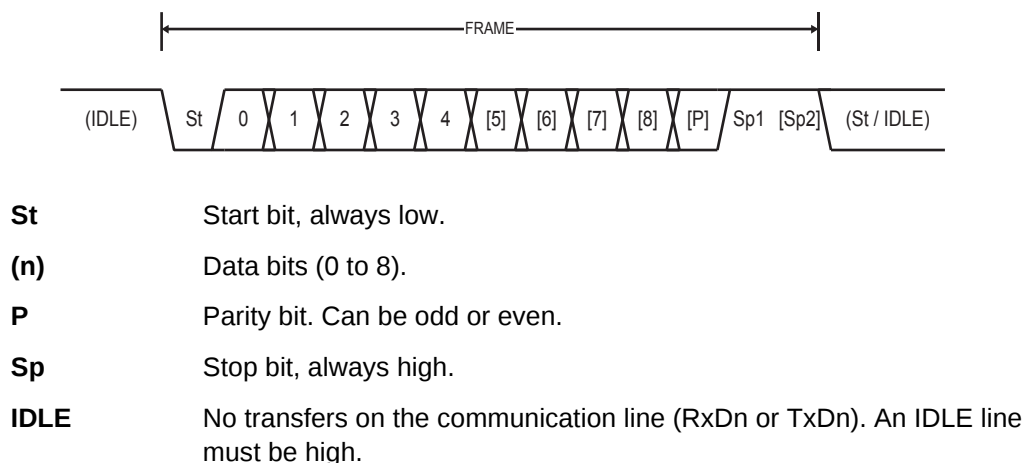
Figure 16-4. Frame Formats
