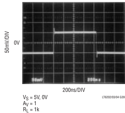
5V Small-Signal Response
