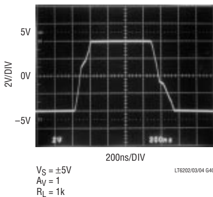
±5V Large-Signal Response
