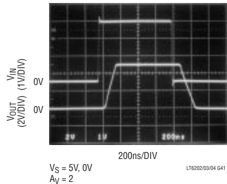
Output-Overdrive Recovery
