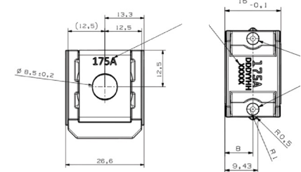
Dimensions [mm]
