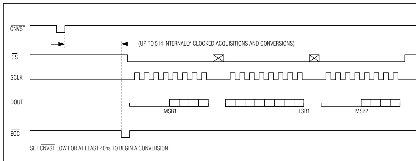
Figure 4. Clock Mode 00
