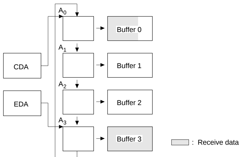
Figure 6.21 MSCI-to-Memory Chained-Block Multi-Frame Transfer (part of a buffer released during reception operation)
