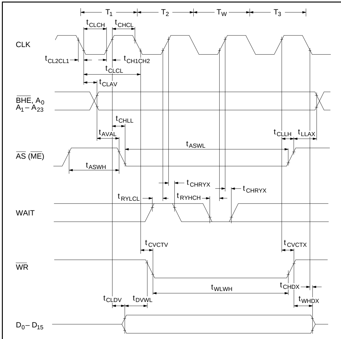
Figure 10.6 Master Mode Write Timing (CPU Mode 0) (SCA \neq Memory)
